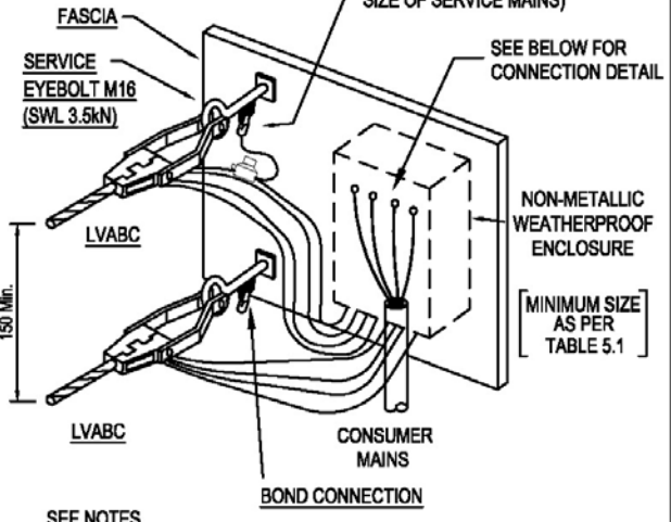
TYPICAL LVABC TO PARALLEL SERVICES MAINS CONNECTION DETAIL
