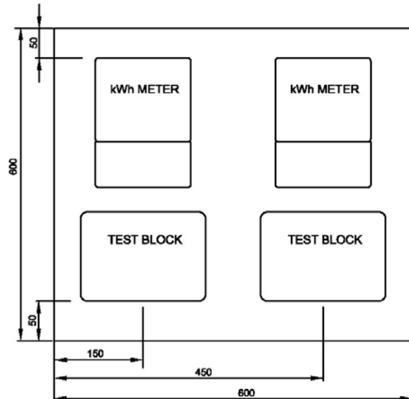
TYPICAL LAYOUT FOR SINGLE NMI CT. METERING
